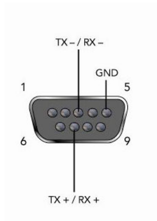
Figure 2-7. RS-485 2-Wire Pinouts
